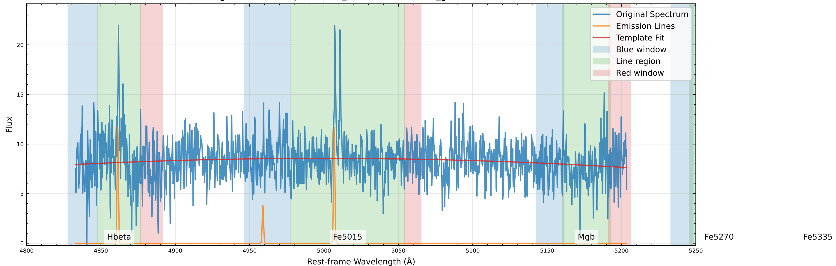
Original Data Comparison (v_star=-27.4 km/s, v_gas=29.3 km/s)
