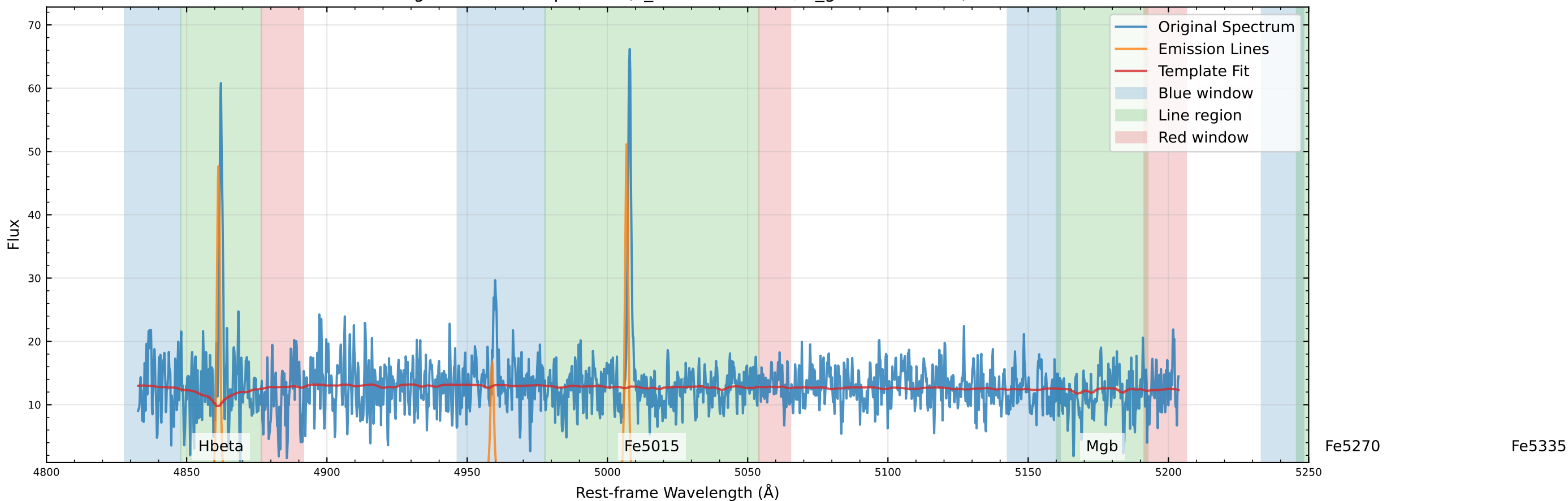
Original Data Comparison (v_star=38.2 km/s, v_gas=59.6 km/s)
