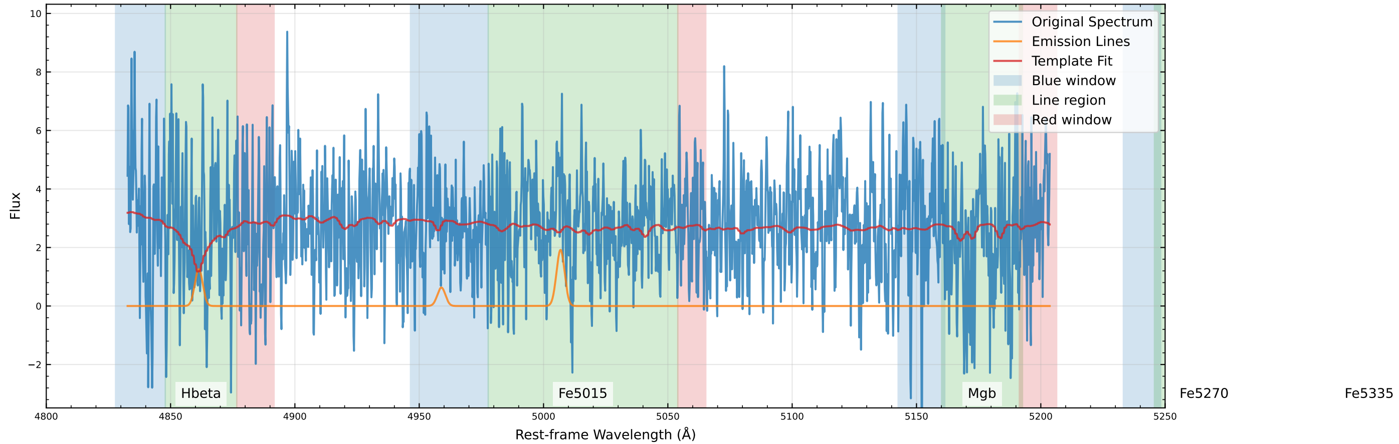
Original Data Comparison (v_star=-31.1 km/s, v_gas=-31.3 km/s)
