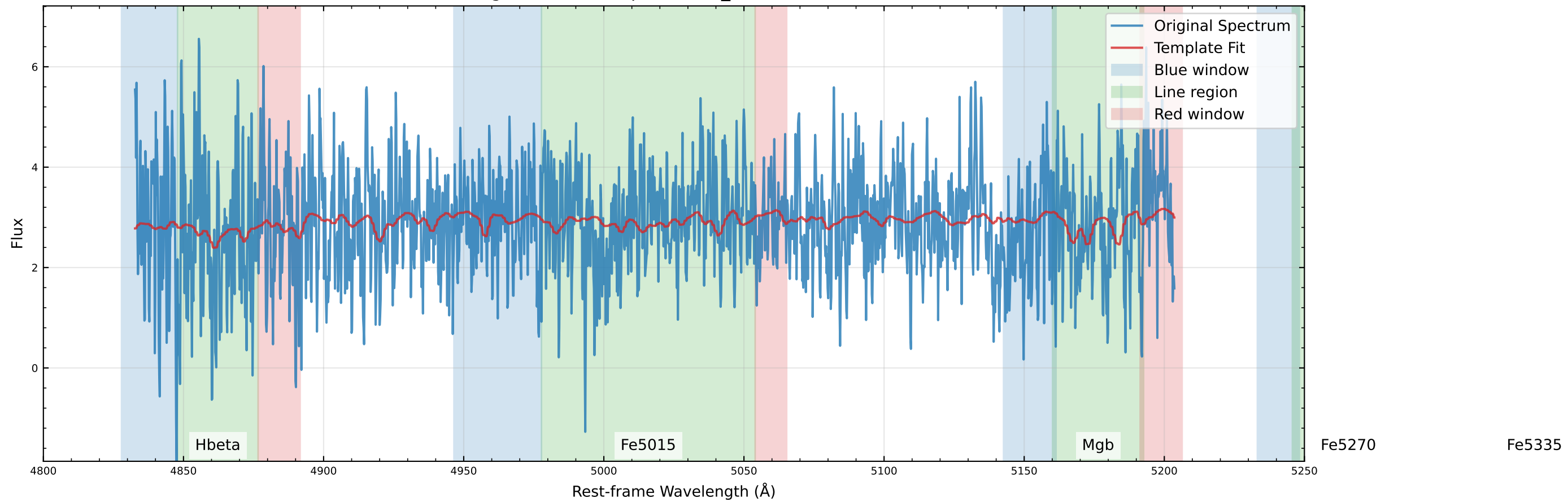
Original Data Comparison (v_star=-71.4 km/s)
