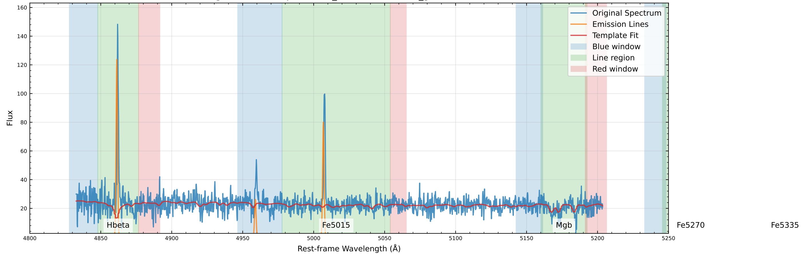
Original Data Comparison (v_star=64.2 km/s, v_gas=41.7 km/s)
