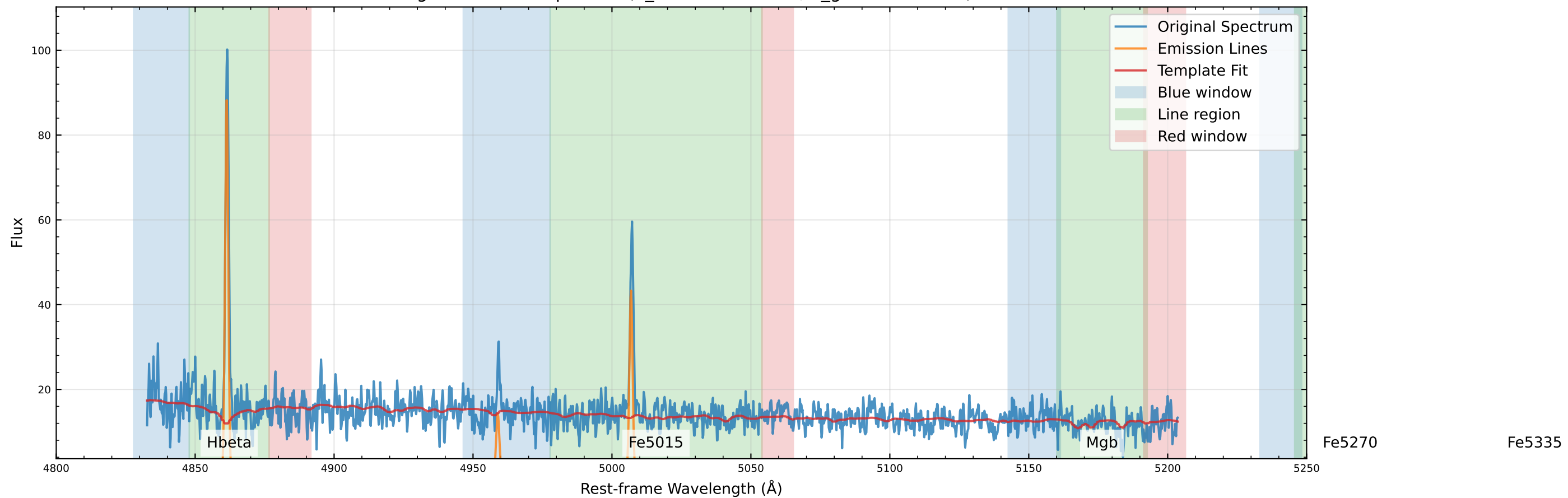
Original Data Comparison (v_star=-18.4 km/s, v_gas=13.2 km/s)
