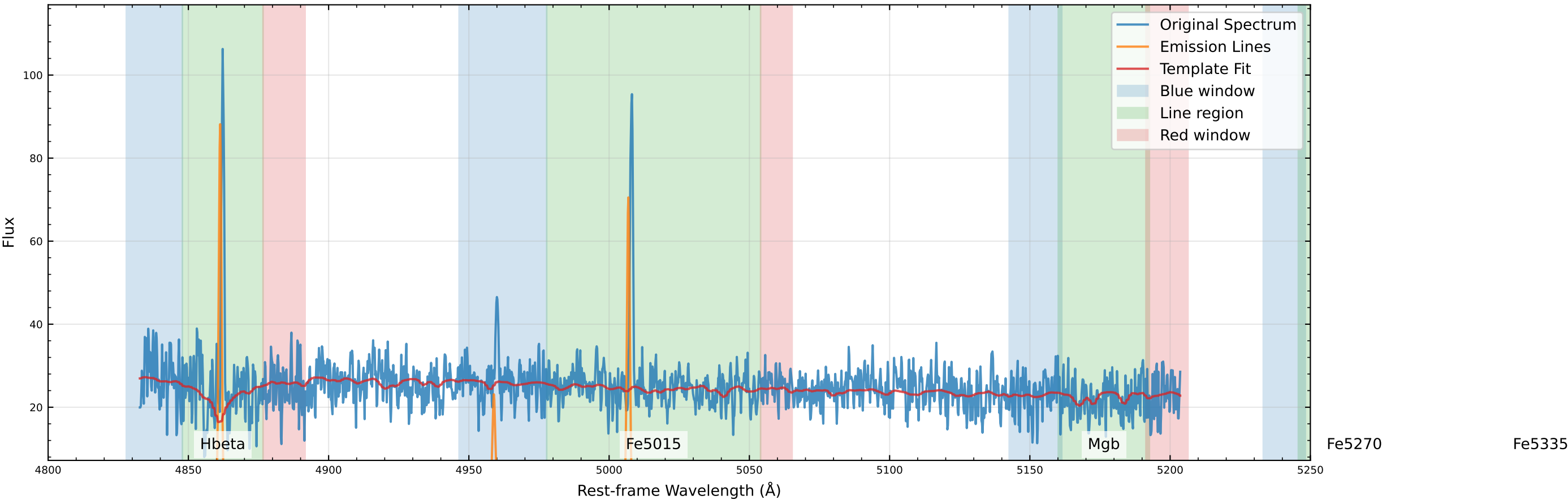
Original Data Comparison (v_star=36.3 km/s, v_gas=61.3 km/s)
