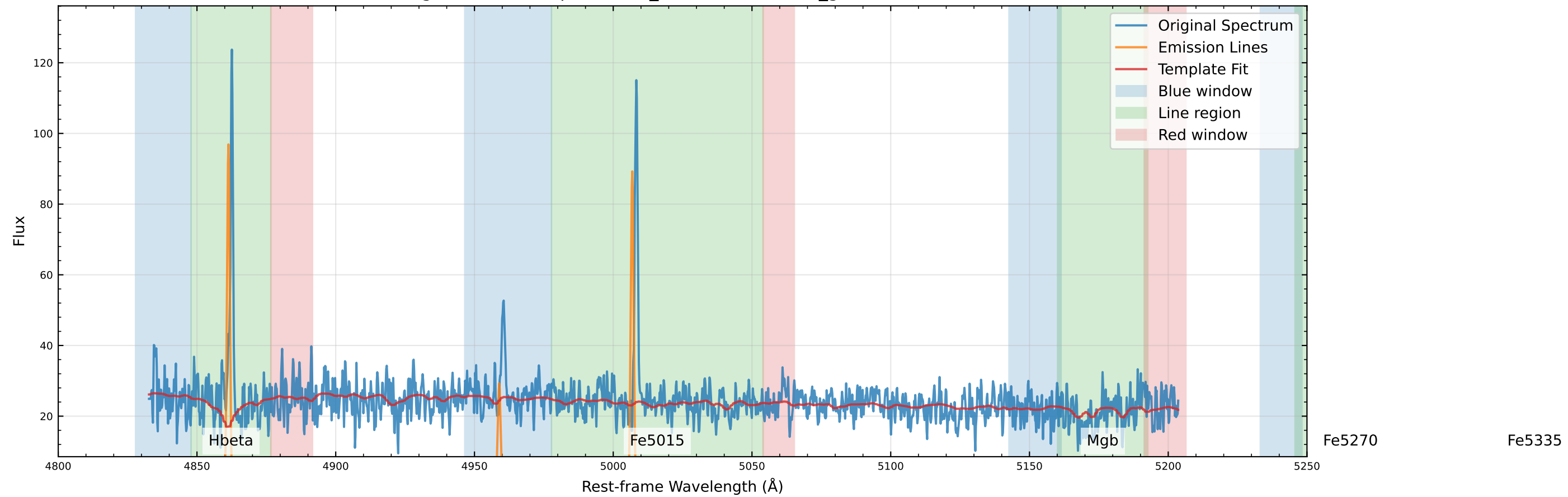
Original Data Comparison (v_star=82.5 km/s, v_gas=80.5 km/s)
