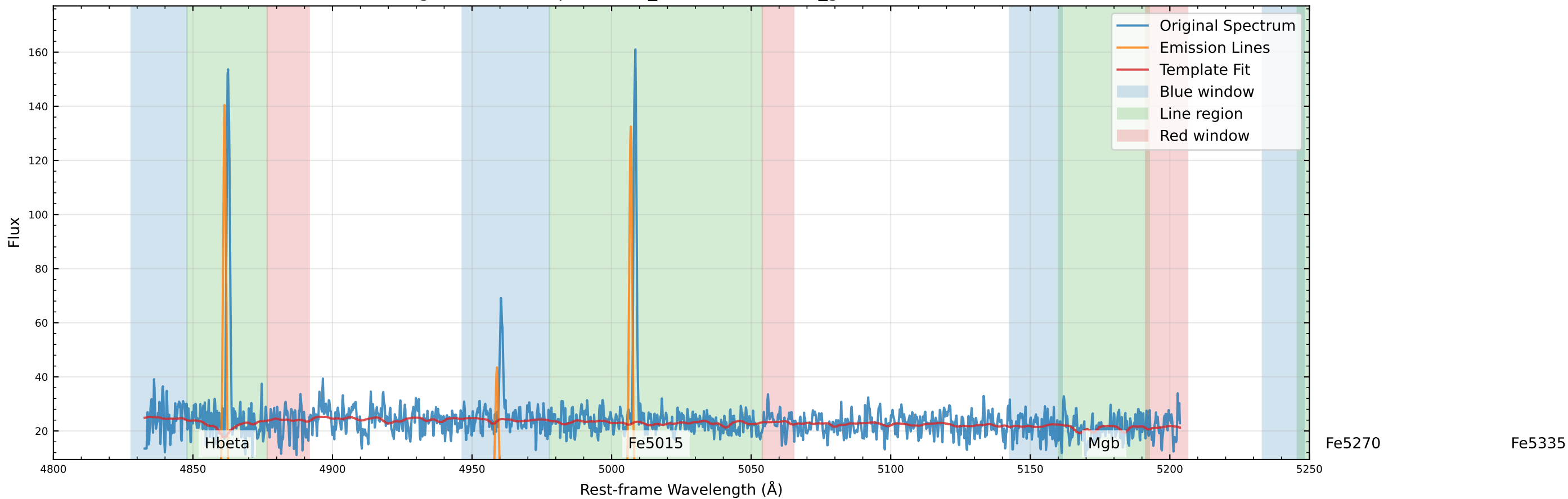
Original Data Comparison (v_star=86.6 km/s, v_gas=87.4 km/s)
