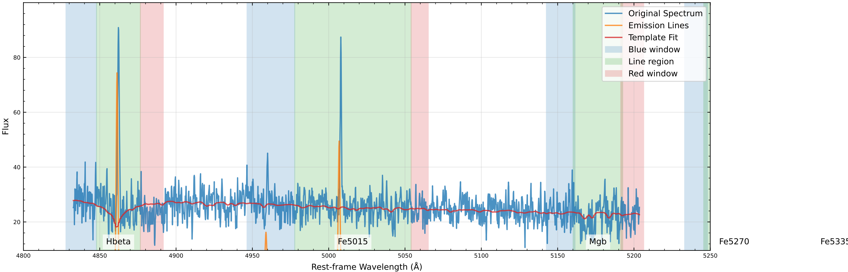
Original Data Comparison (v_star=37.2 km/s, v_gas=60.4 km/s)
