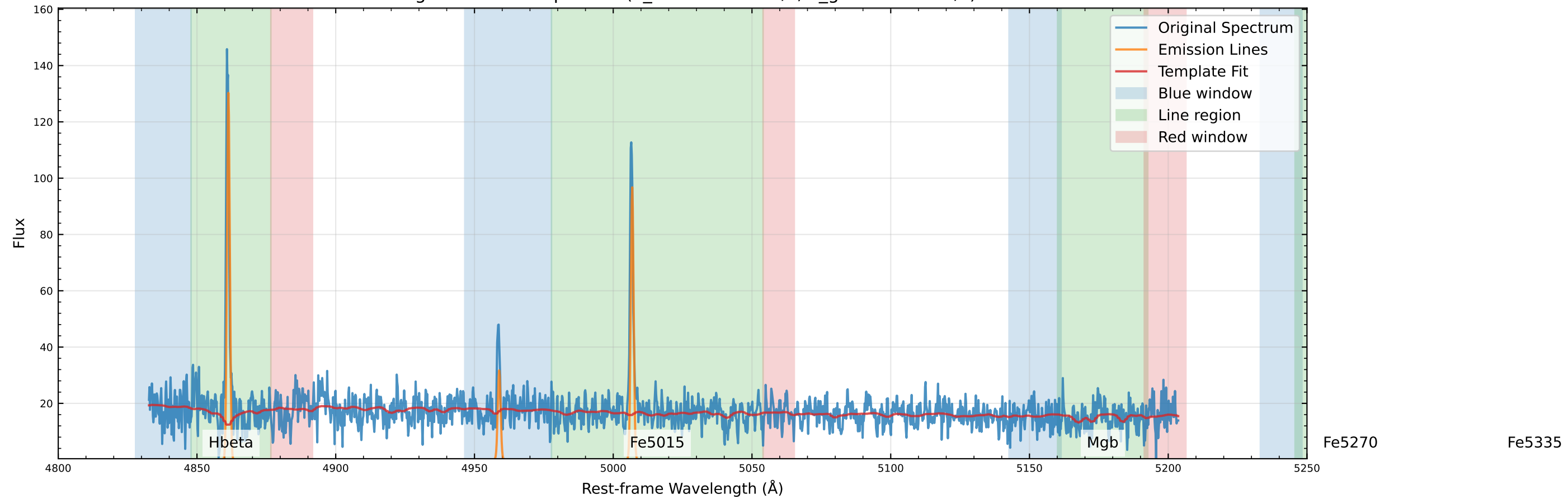
Original Data Comparison (v_star=-46.9 km/s, v_gas=-20.3 km/s)
