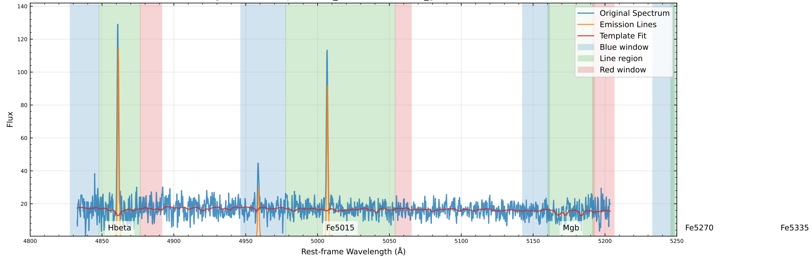
Original Data Comparison (v_star=-46.2 km/s, v_gas=-17.2 km/s)
