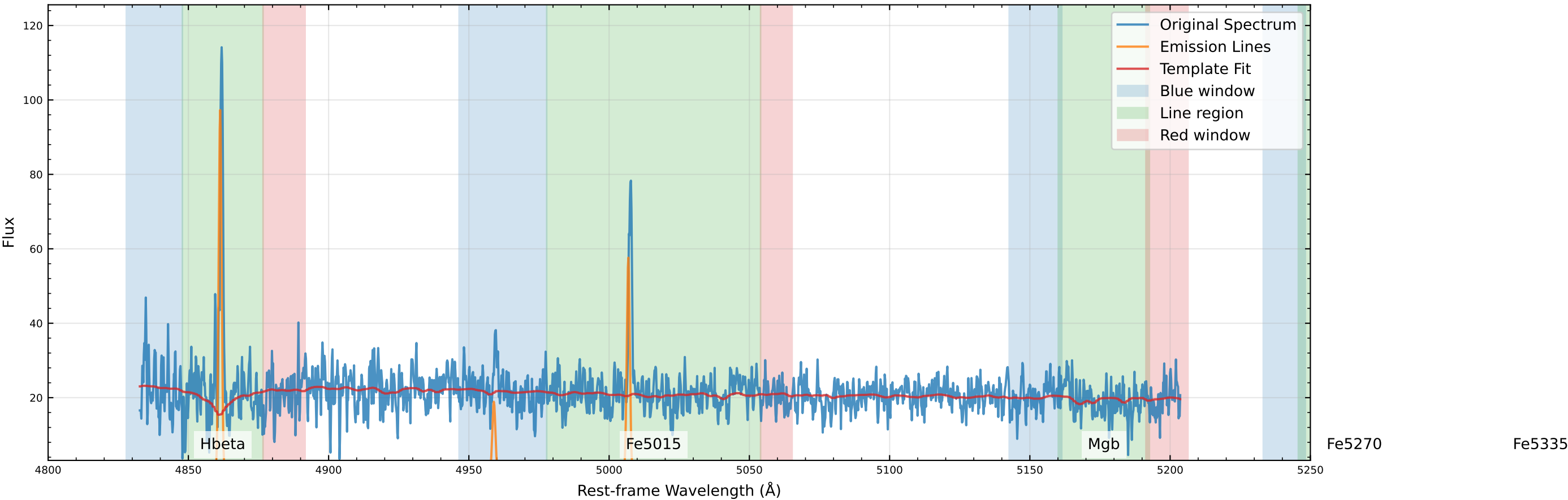
Original Data Comparison (v_star=47.8 km/s, v_gas=35.2 km/s)
