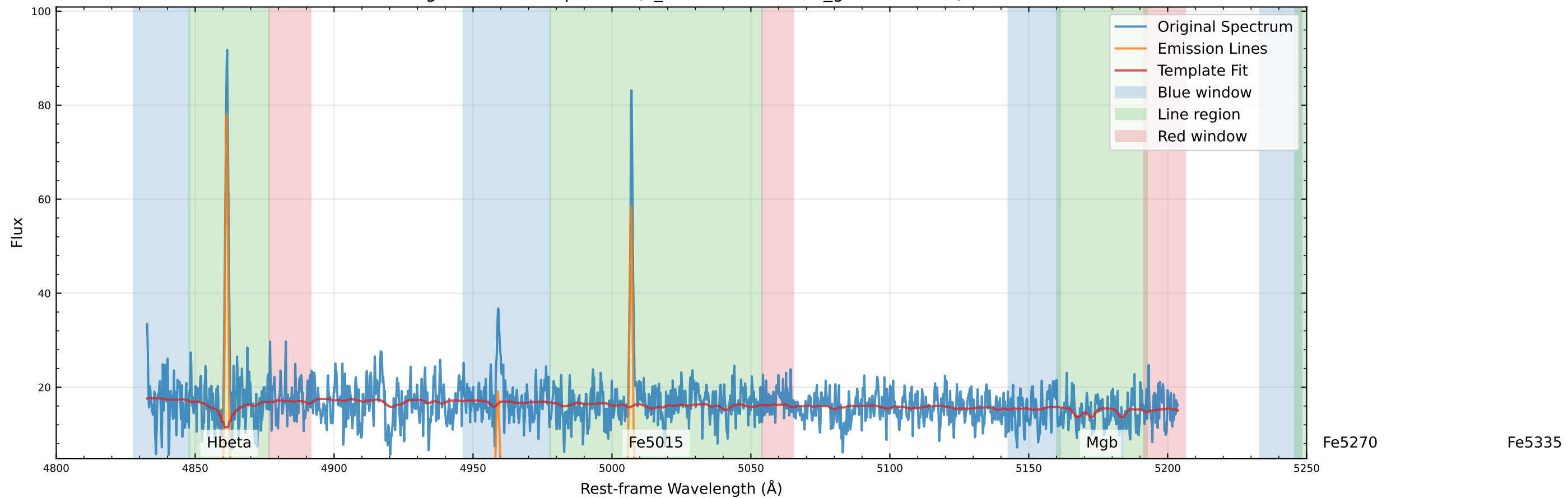
Original Data Comparison (v_star=16.1 km/s, v_gas=7.6 km/s)
