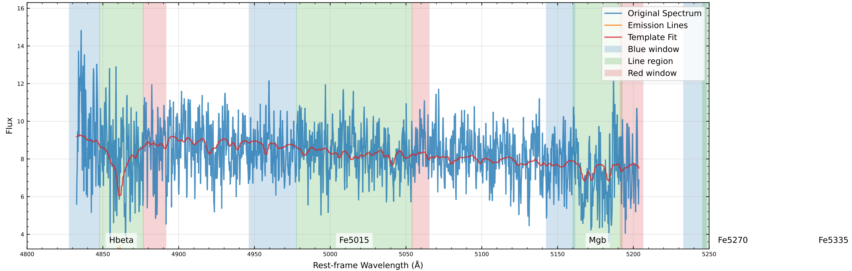
Original Data Comparison (v_star=16.3 km/s, v_gas=65.5 km/s)
