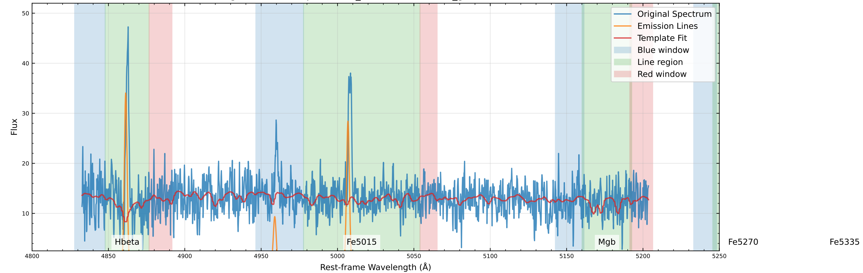
Original Data Comparison (v_star=-23.4 km/s, v_gas=73.4 km/s)
