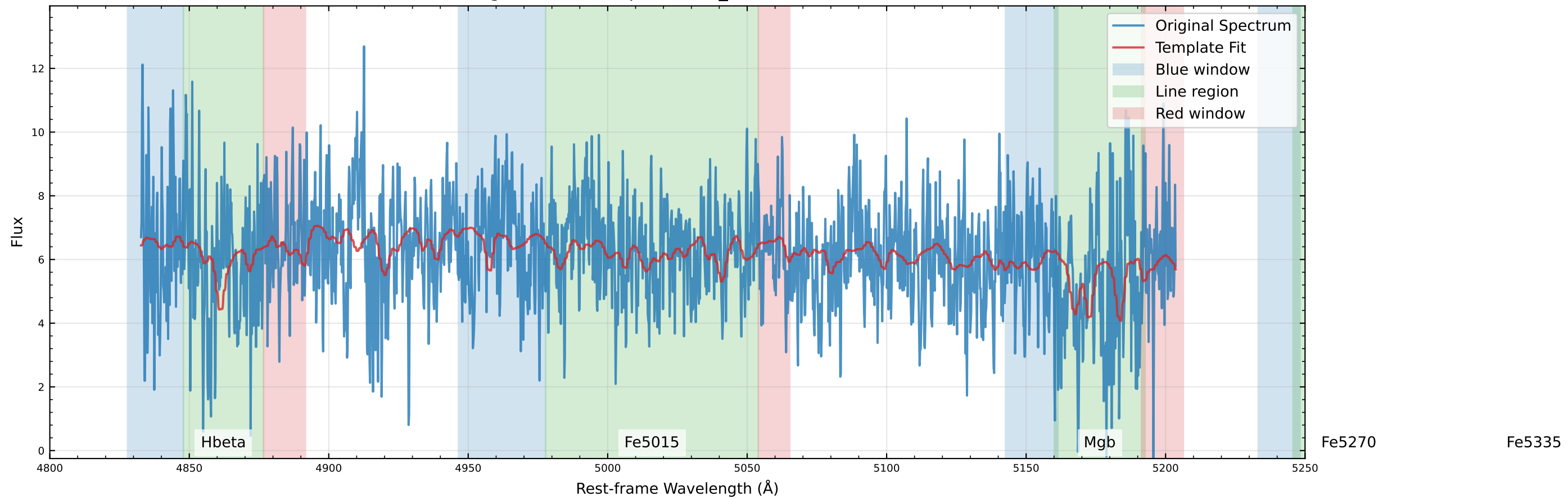
Original Data Comparison (v_star=-257.6 km/s)
