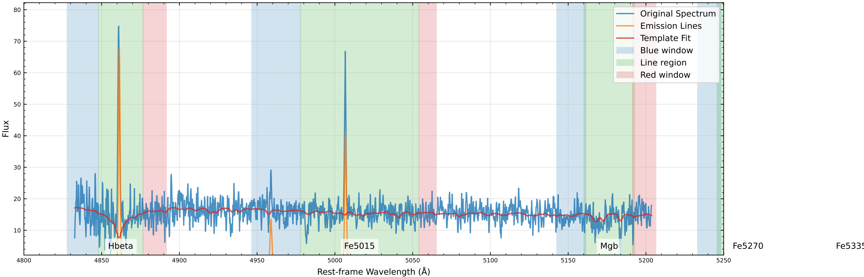
Original Data Comparison (v_star=-23.3 km/s, v_gas=-17.1 km/s)
