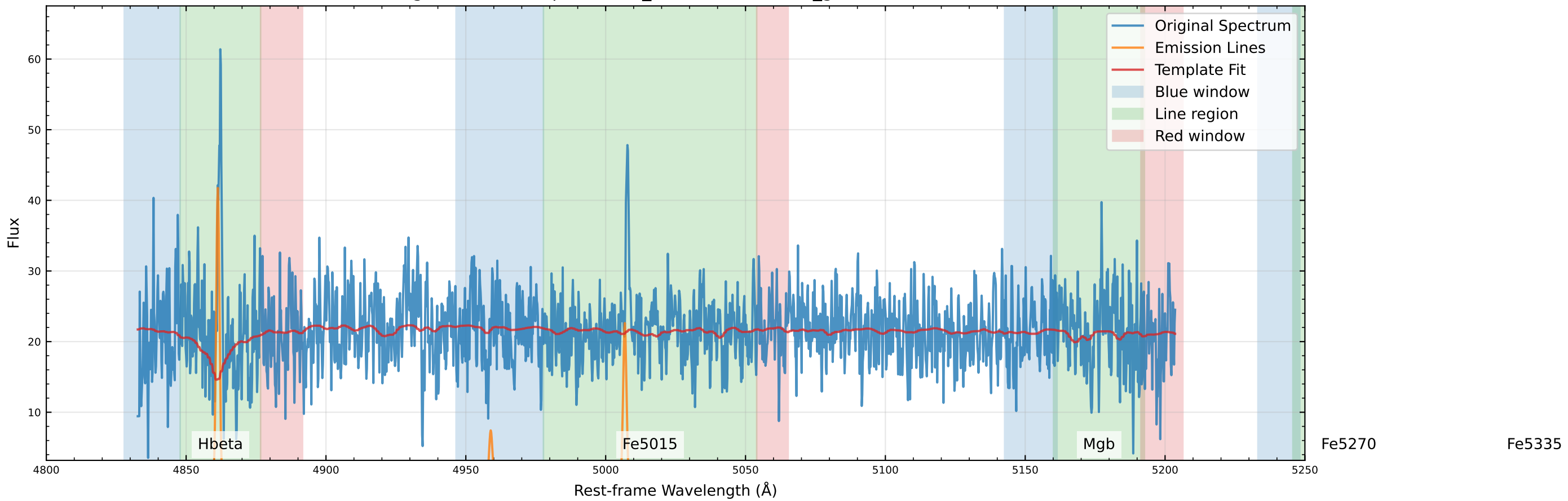
Original Data Comparison (v_star=64.9 km/s, v_gas=49.1 km/s)
