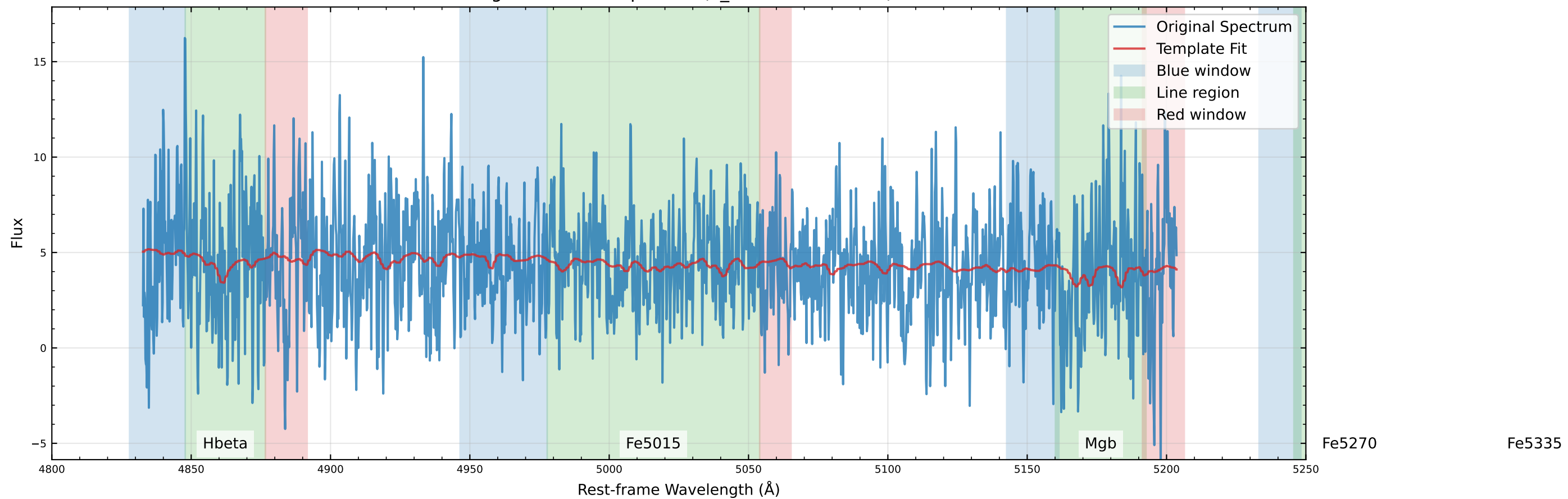
Original Data Comparison (v_star=-133.1 km/s)
