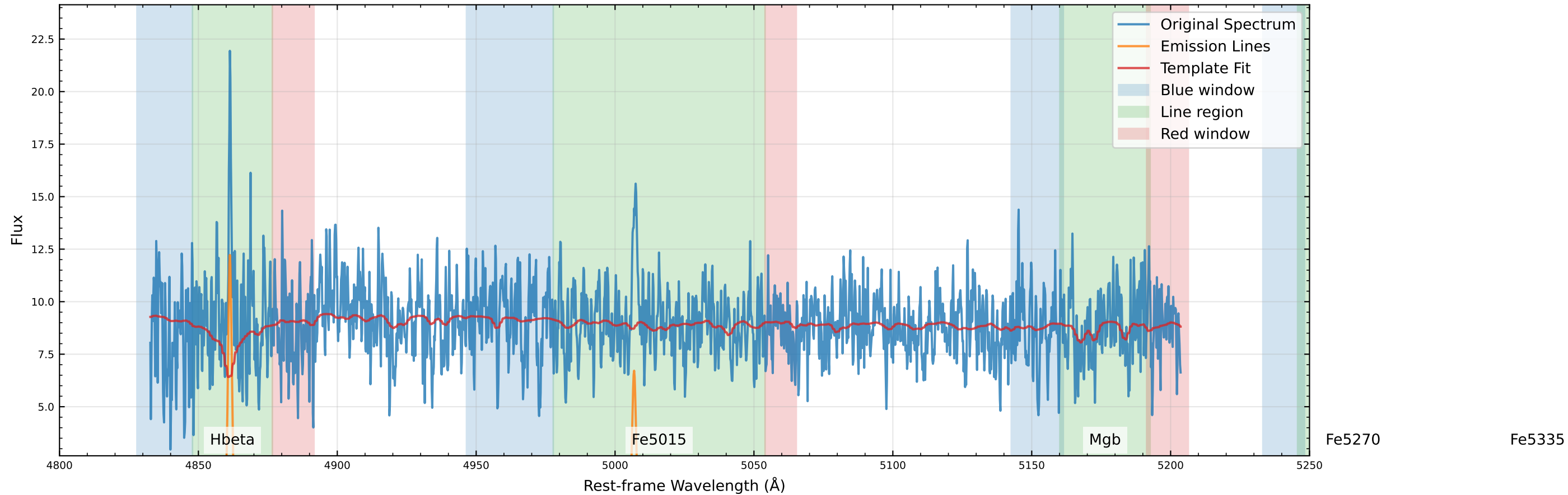
Original Data Comparison (v_star=18.6 km/s, v_gas=10.6 km/s)
