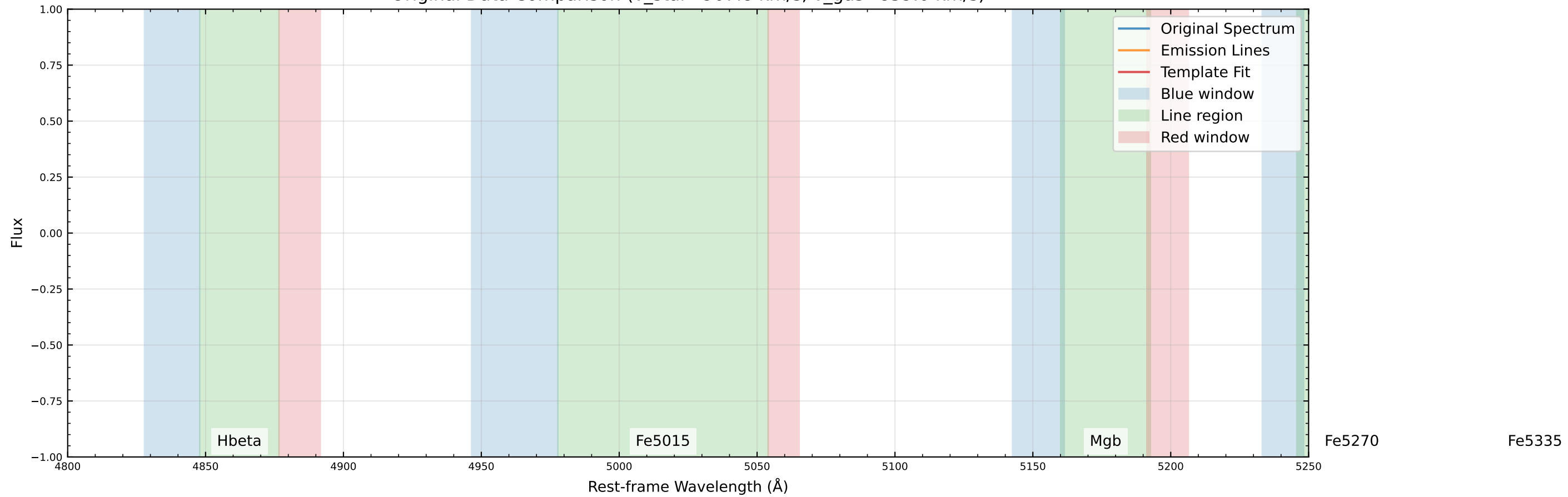
Original Data Comparison (v_star=907.8 km/s, v_gas=839.0 km/s)
