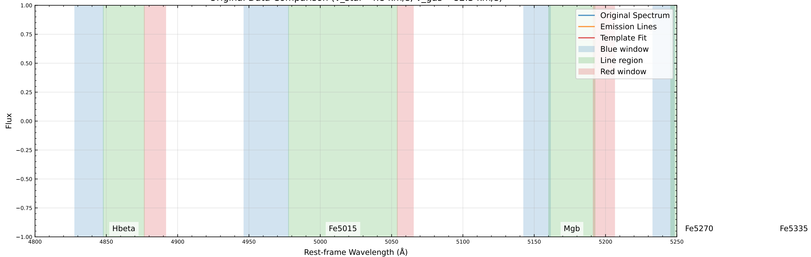
Original Data Comparison (v_star=4.8 km/s, v_gas=-82.3 km/s)
