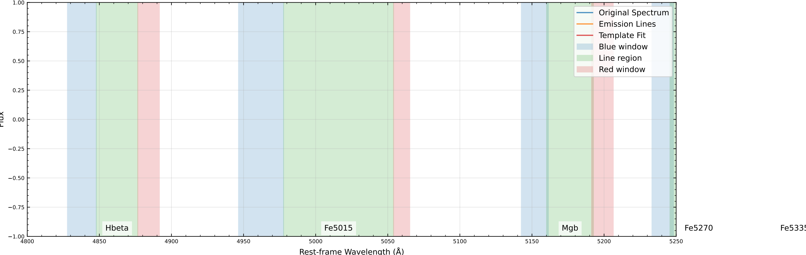
Original Data Comparison (v_star=793.0 km/s)
