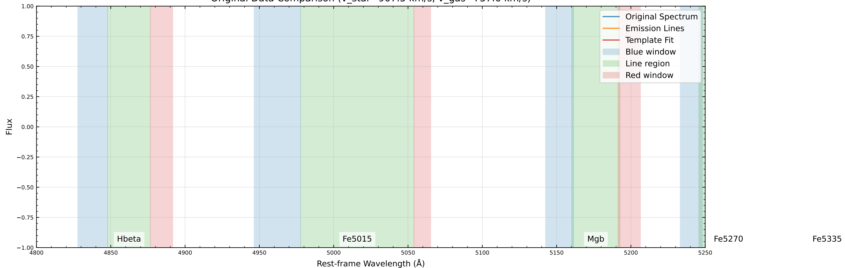
Original Data Comparison (v_star=907.5 km/s, v_gas=737.6 km/s)
