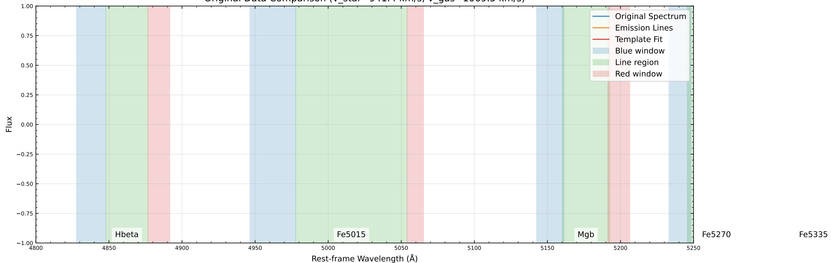
Original Data Comparison (v_star=941.4 km/s, v_gas=1069.5 km/s)
