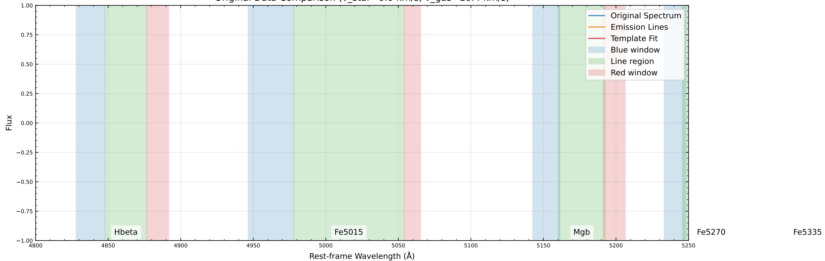
Original Data Comparison (v_star=0.0 km/s, v_gas=10.4 km/s)
