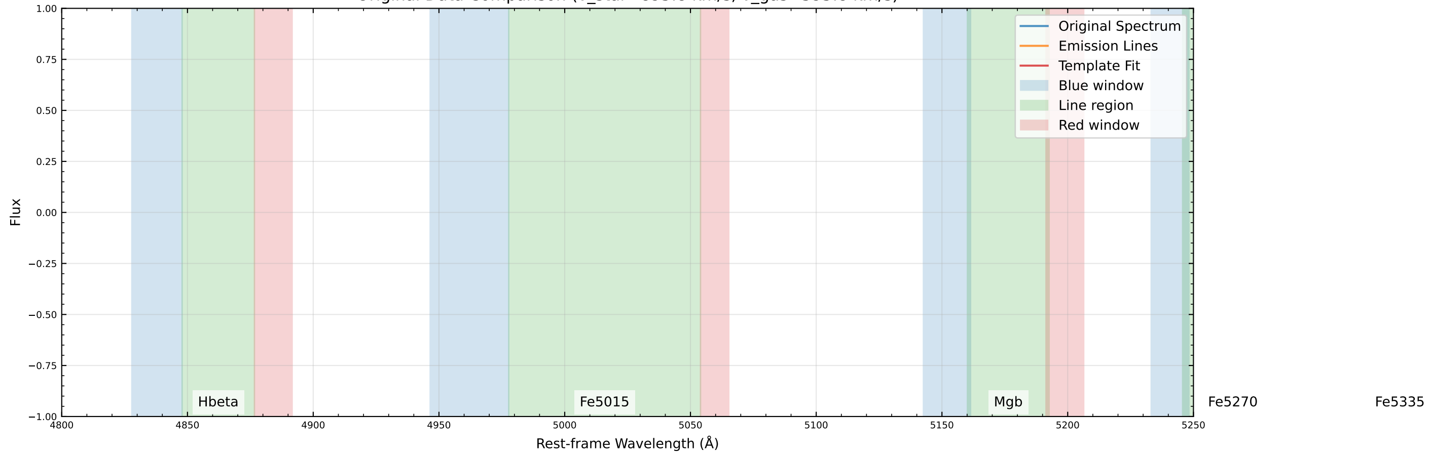
Original Data Comparison (v_star=895.8 km/s, v_gas=595.8 km/s)
