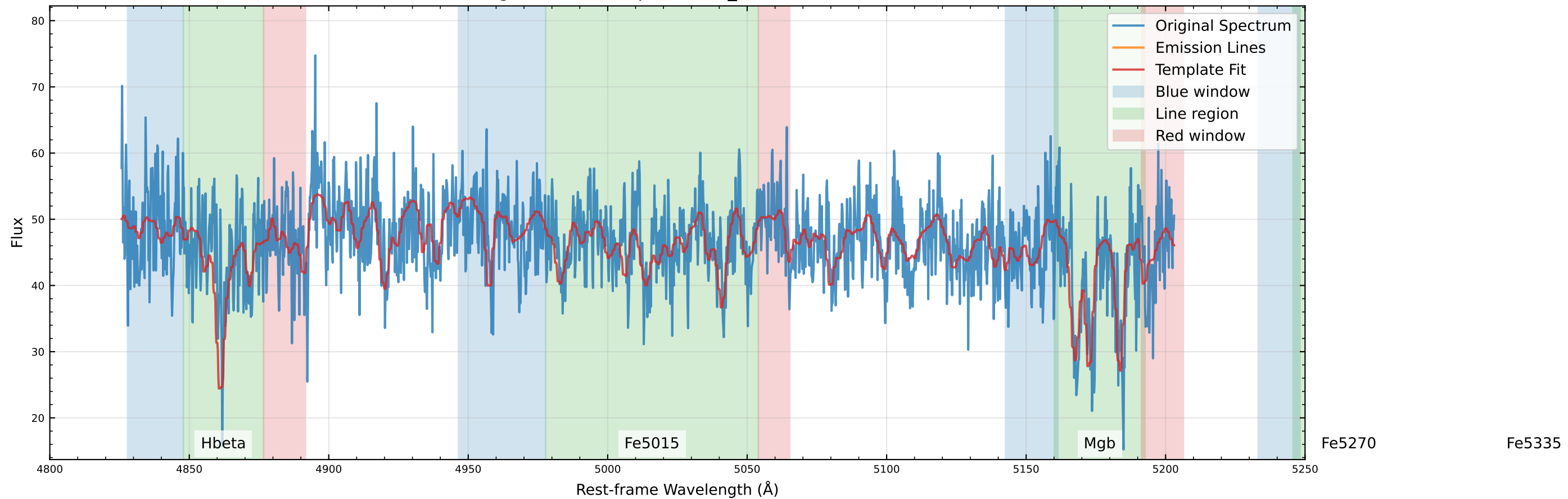
Original Data Comparison (v_star=42.5 km/s)
