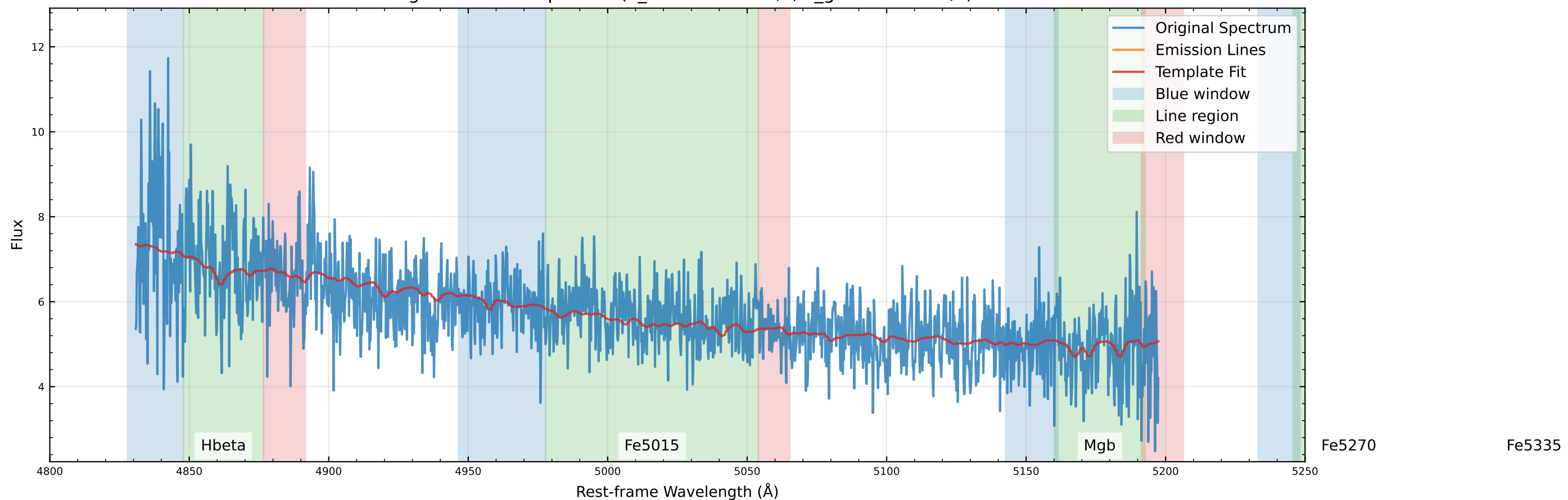
Original Data Comparison (v_star=-34.3 km/s, v_gas=-34.6 km/s)
