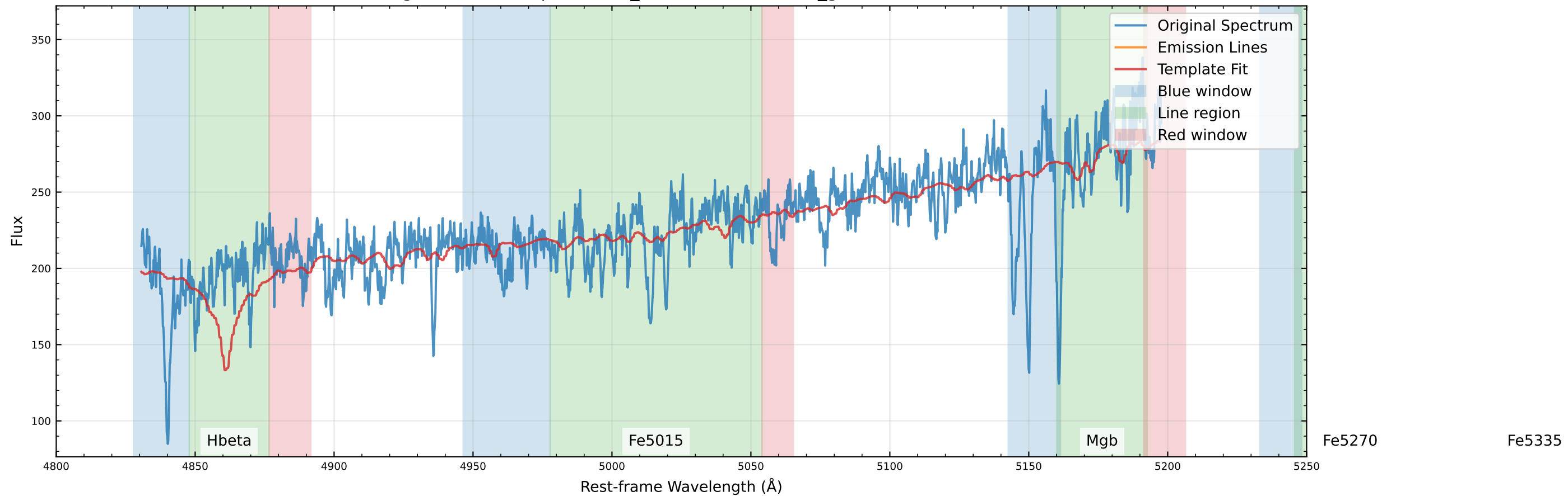
Original Data Comparison (v_star=-329.6 km/s, v_gas=-308.2 km/s)
