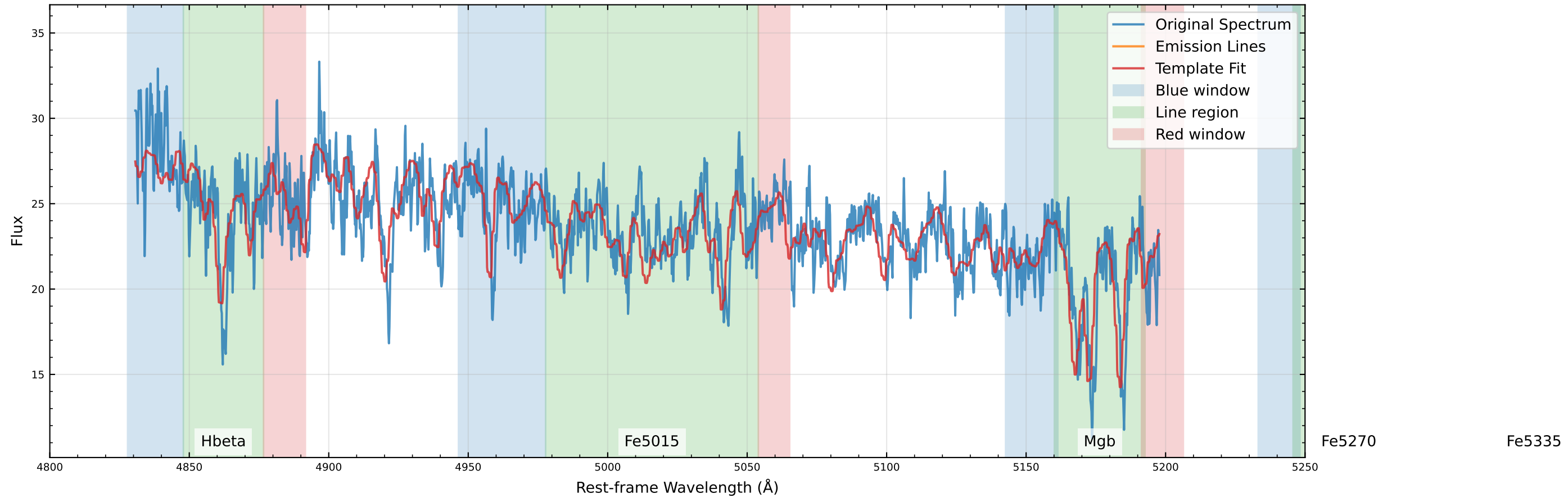
Original Data Comparison ( v_{\text{star}}=74.5 km/s, v_{\text{gas}}=116.6 km/s)
