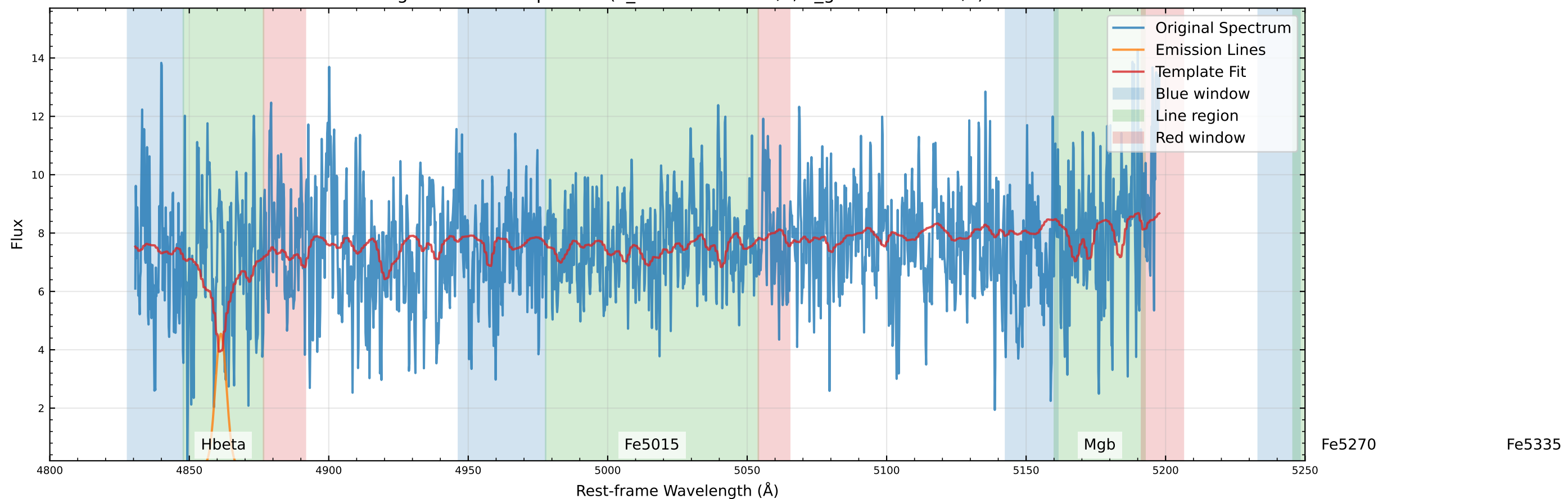
Original Data Comparison ( v_{\text{star}}=-301.8 km/s, v_{\text{gas}}=-351.6 km/s)
