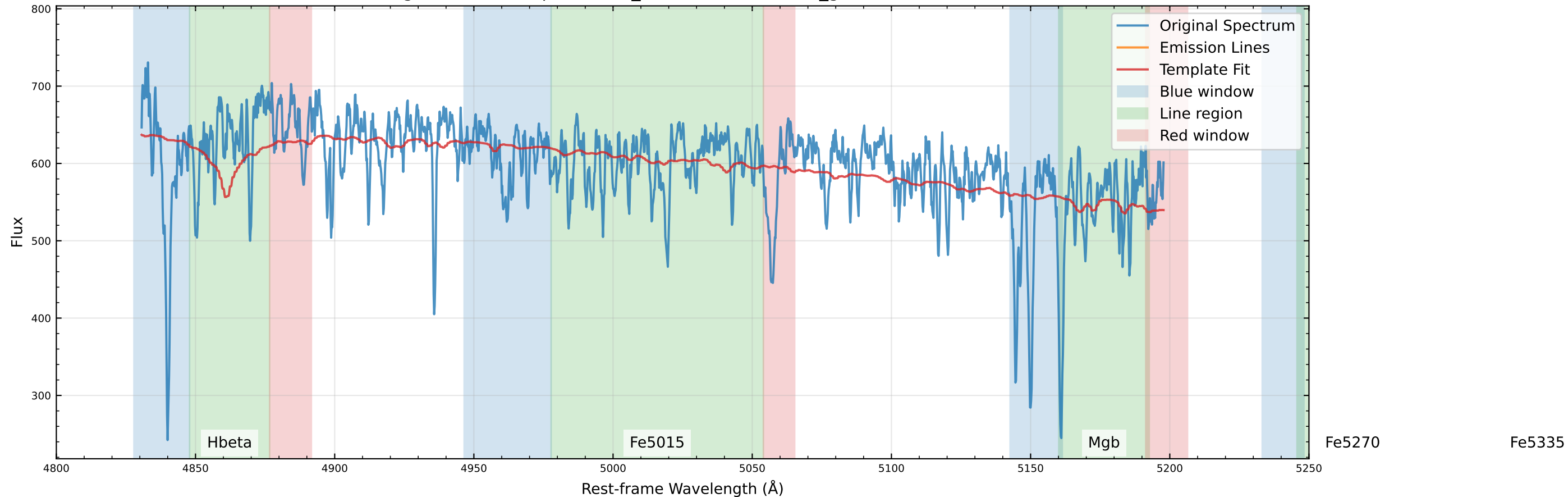
Original Data Comparison (v_star=-404.2 km/s, v_gas=-498.1 km/s)
