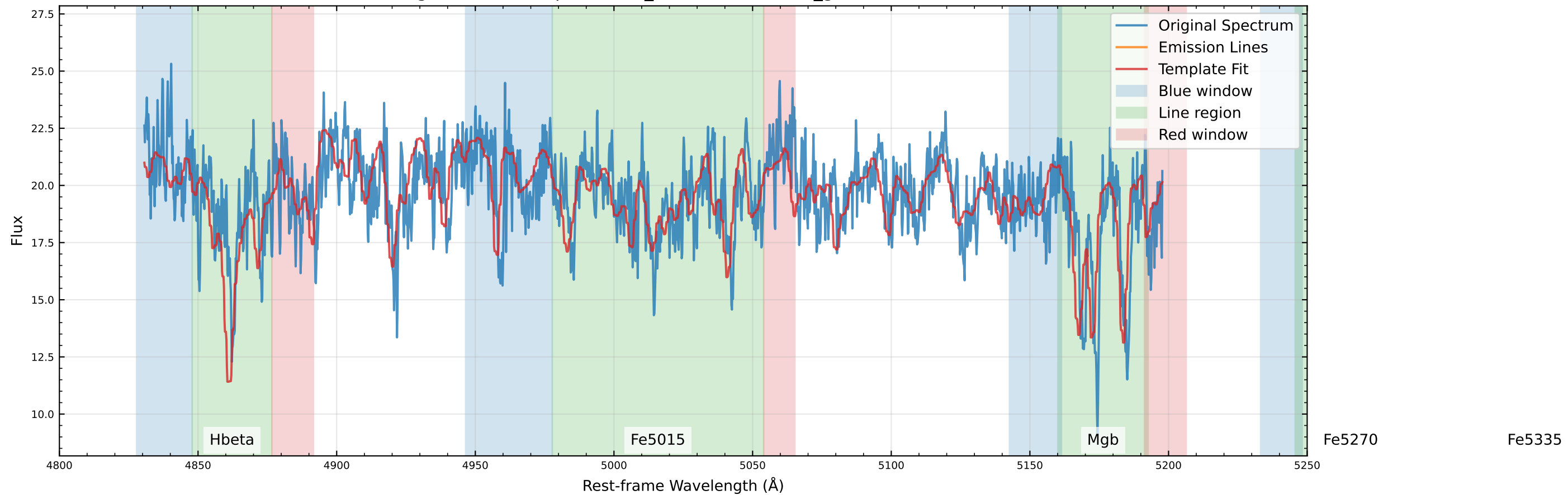
Original Data Comparison (v_star=82.0 km/s, v_gas=119.1 km/s)
