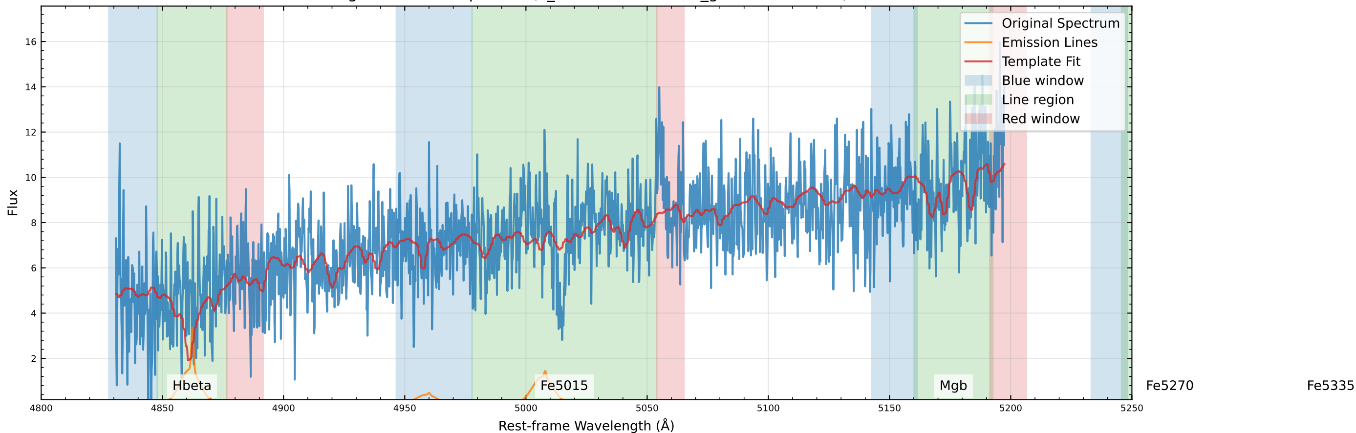
Original Data Comparison (v_star=-97.4 km/s, v_gas=-208.2 km/s)
