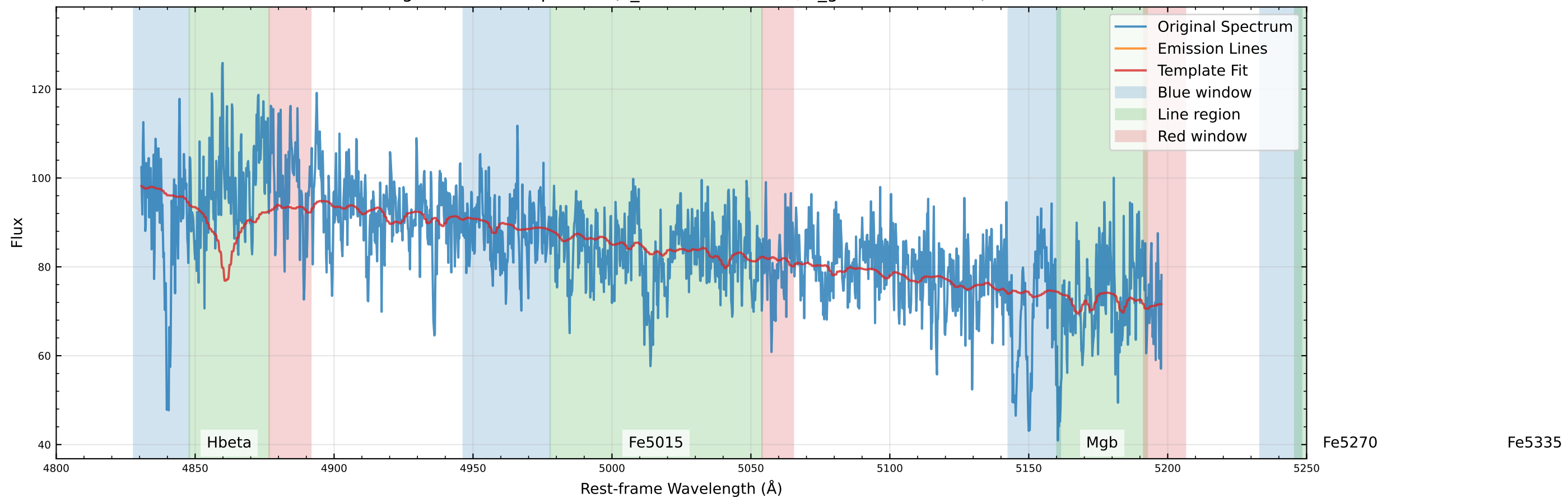
Original Data Comparison (v_star=-135.9 km/s, v_gas=-115.2 km/s)
