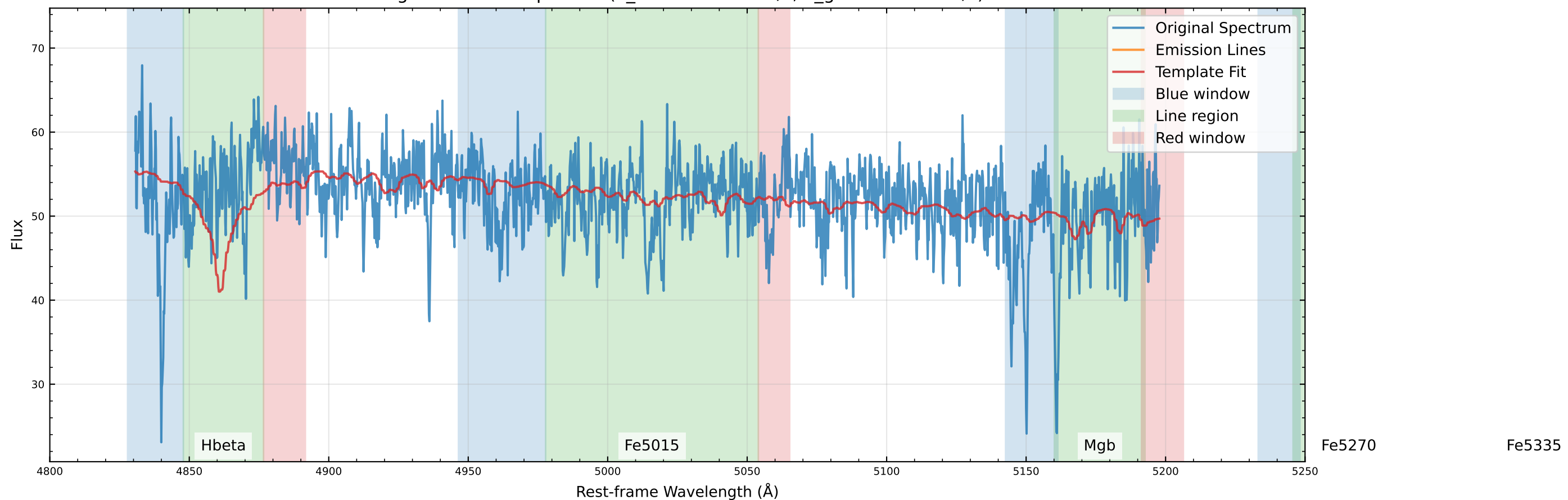
Original Data Comparison (v_star=-344.0 km/s, v_gas=-384.5 km/s)
