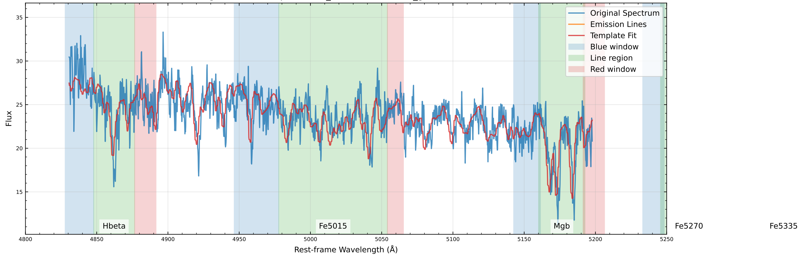
Original Data Comparison (v_star=74.5 km/s, v_gas=116.6 km/s)
