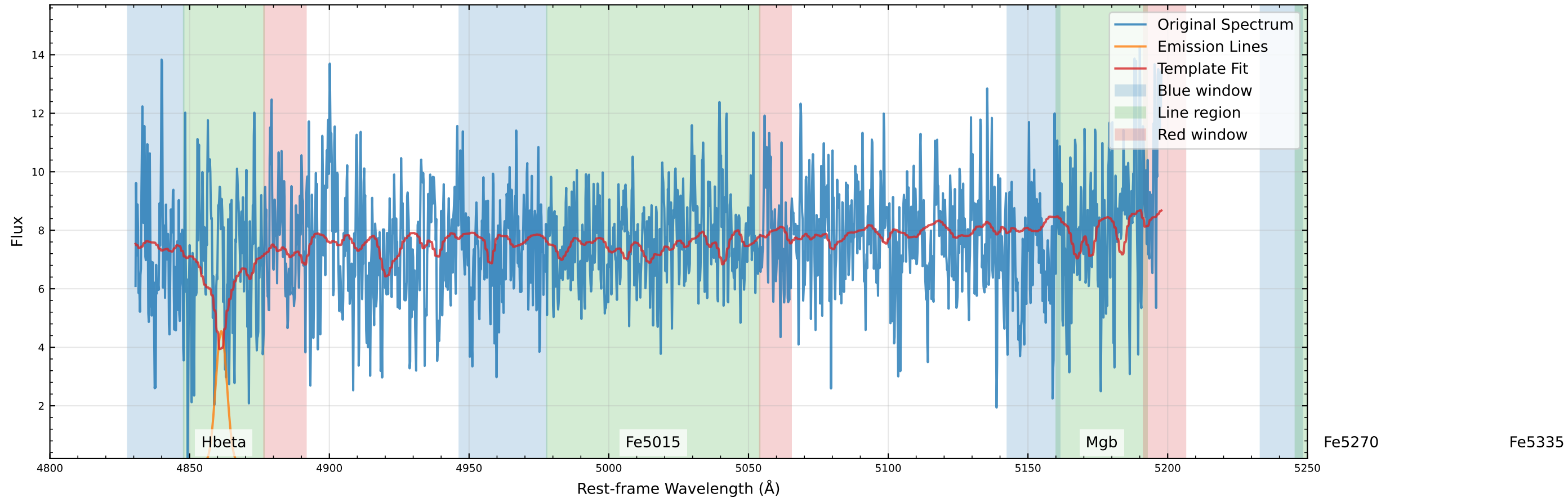
Original Data Comparison (v_star=-301.8 km/s, v_gas=-351.6 km/s)
