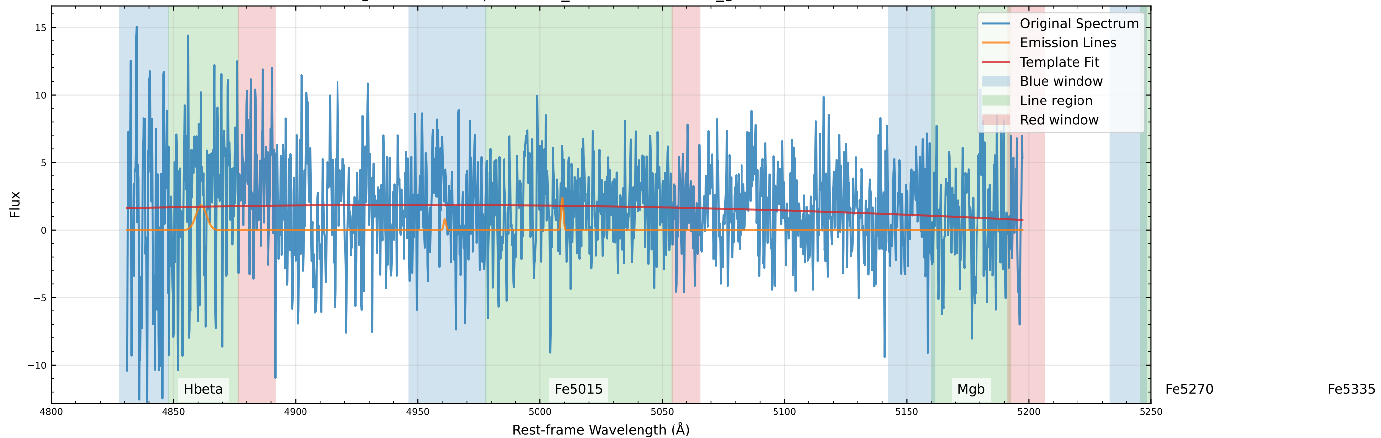
Original Data Comparison (v_star=-51.7 km/s, v_gas=-206.3 km/s)
