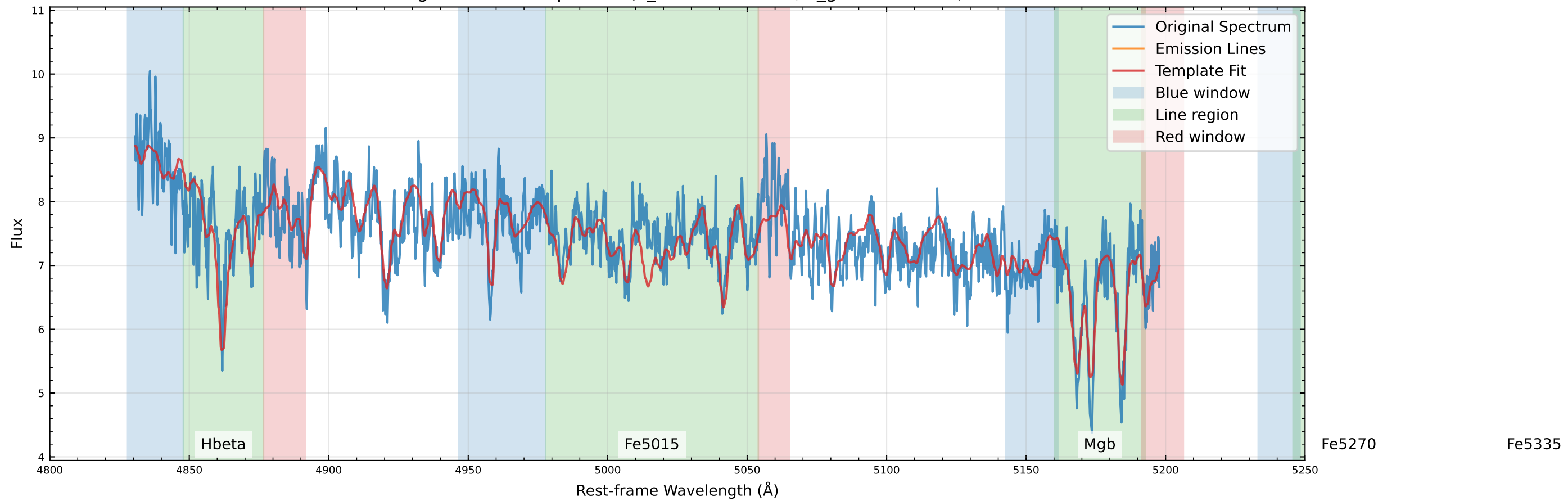
Original Data Comparison (v_star=39.8 km/s, v_gas=-4.5 km/s)
