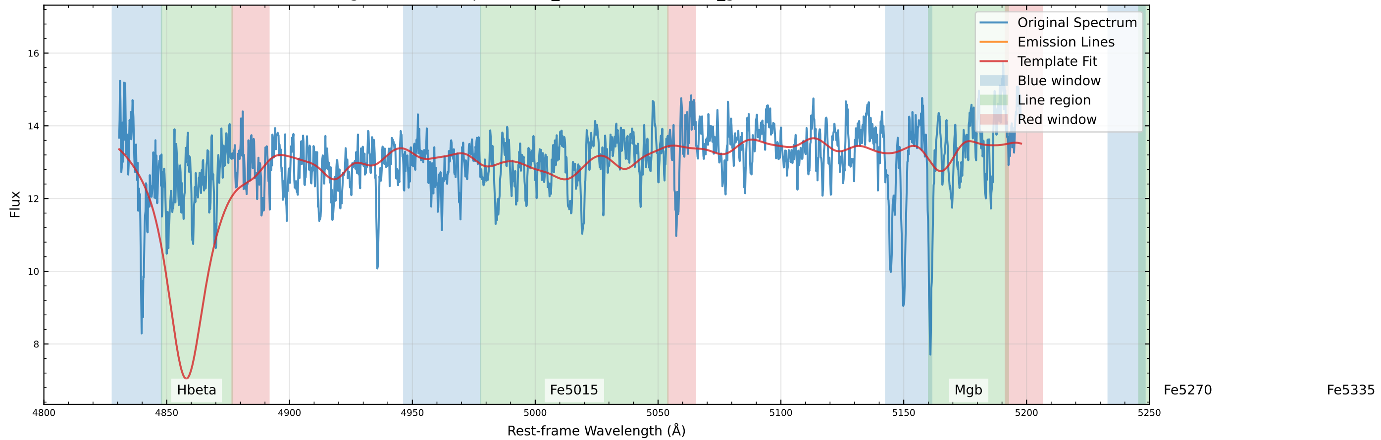
Original Data Comparison (v_star=-203.1 km/s, v_gas=-175.0 km/s)
