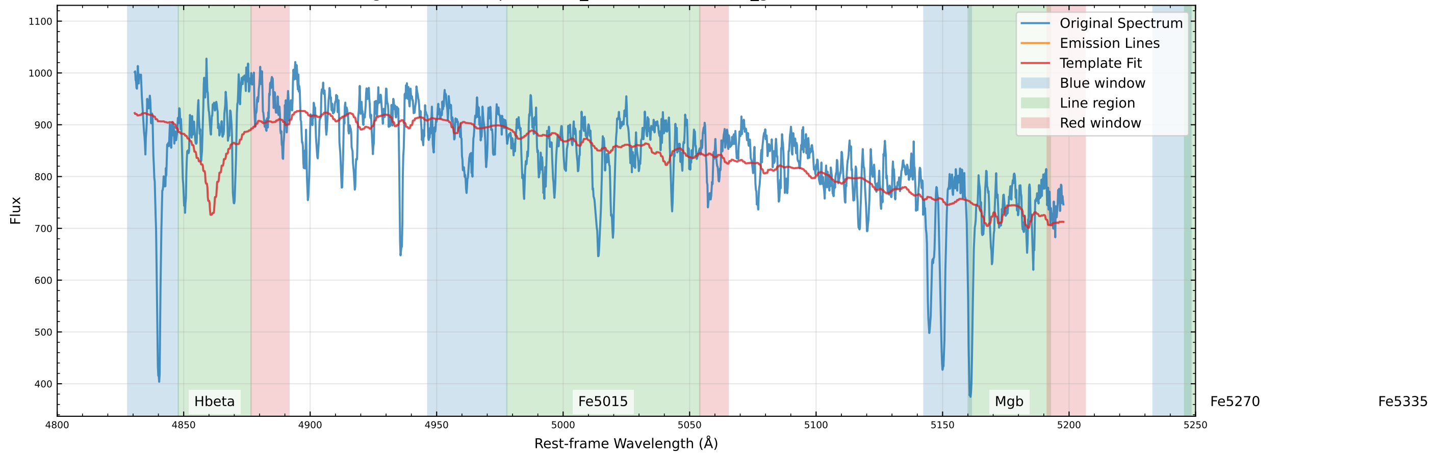
Original Data Comparison (v_star=-371.1 km/s, v_gas=-232.1 km/s)
