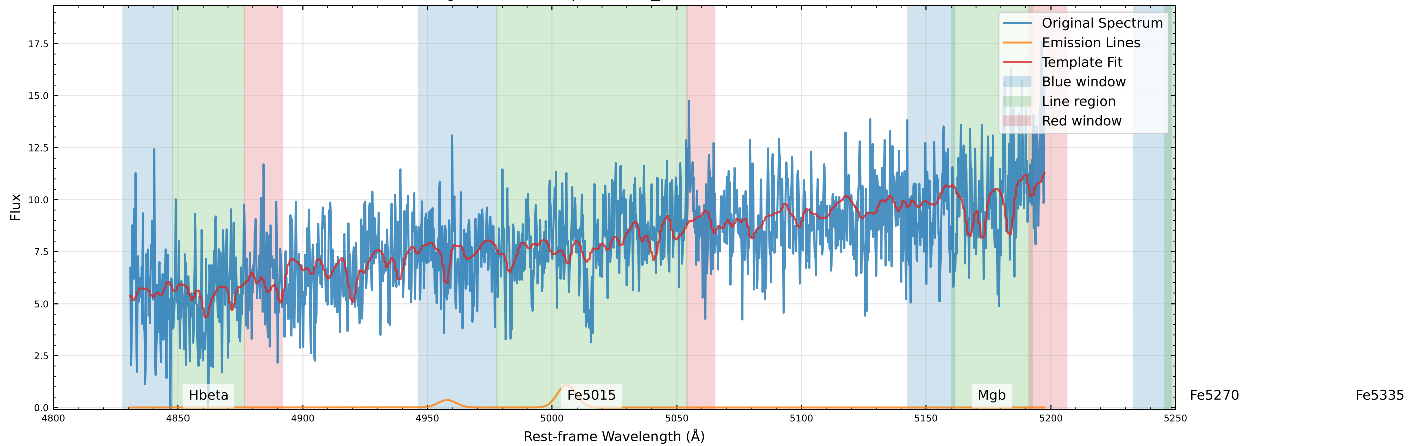
Original Data Comparison (v_star=-207.5 km/s)
