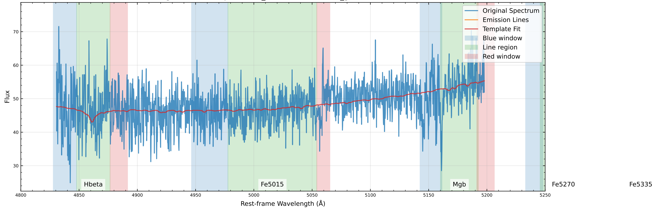
Original Data Comparison (v_star=-371.8 km/s, v_gas=-420.1 km/s)
