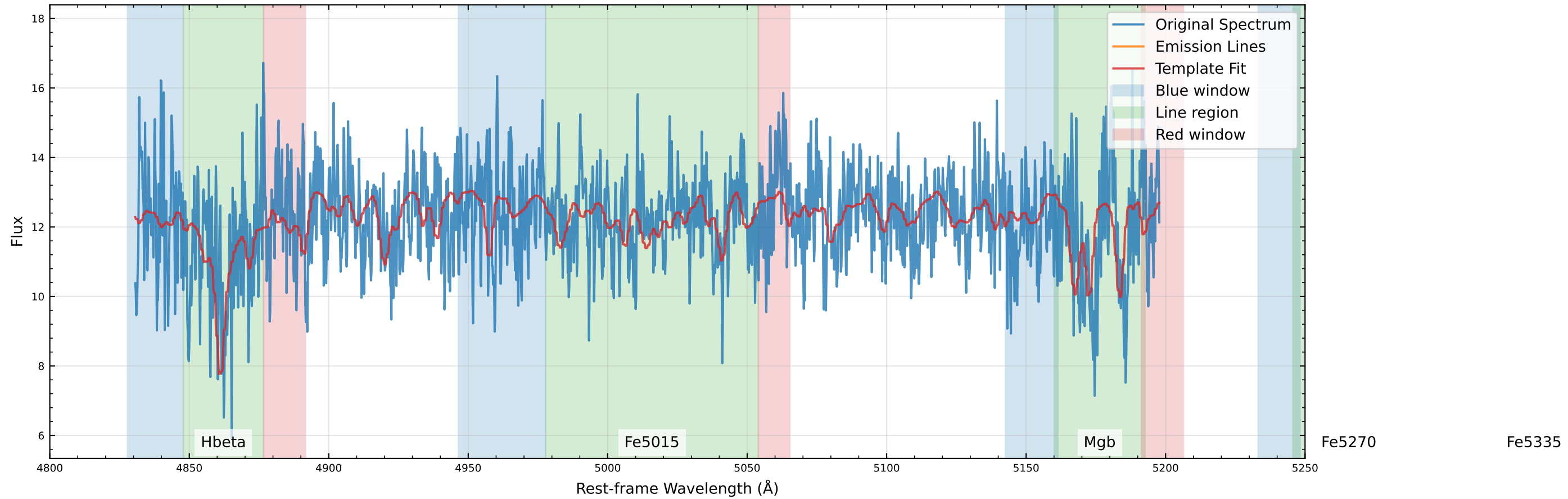
Original Data Comparison (v_star=101.9 km/s, v_gas=134.5 km/s)
