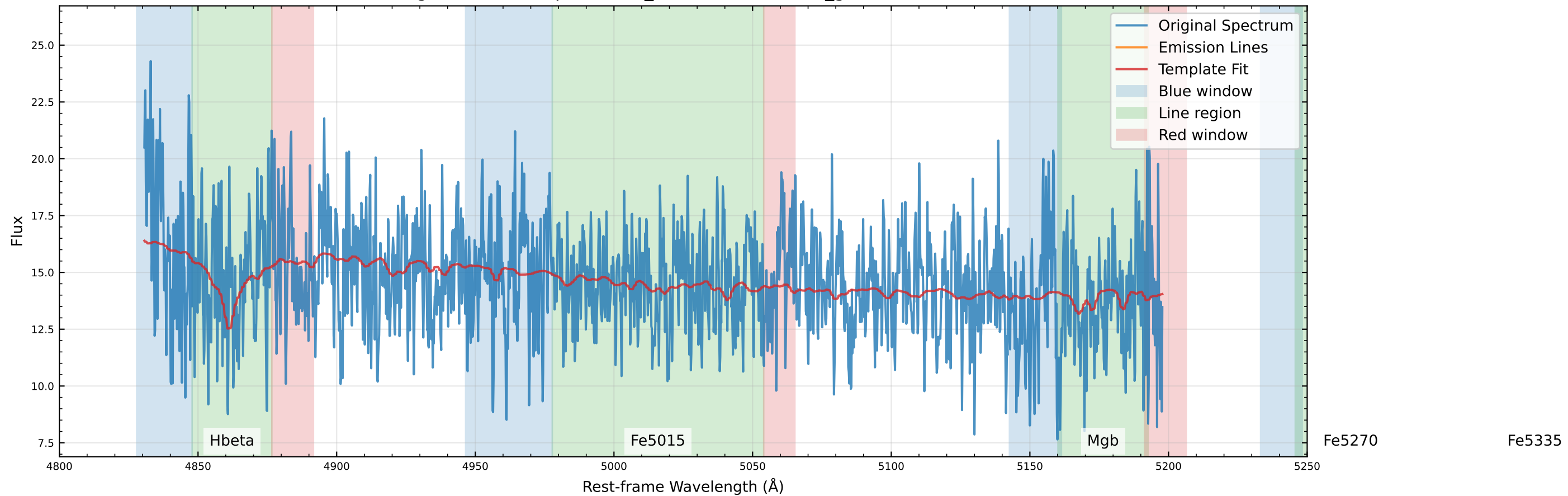
Original Data Comparison (v_star=103.0 km/s, v_gas=16.9 km/s)
