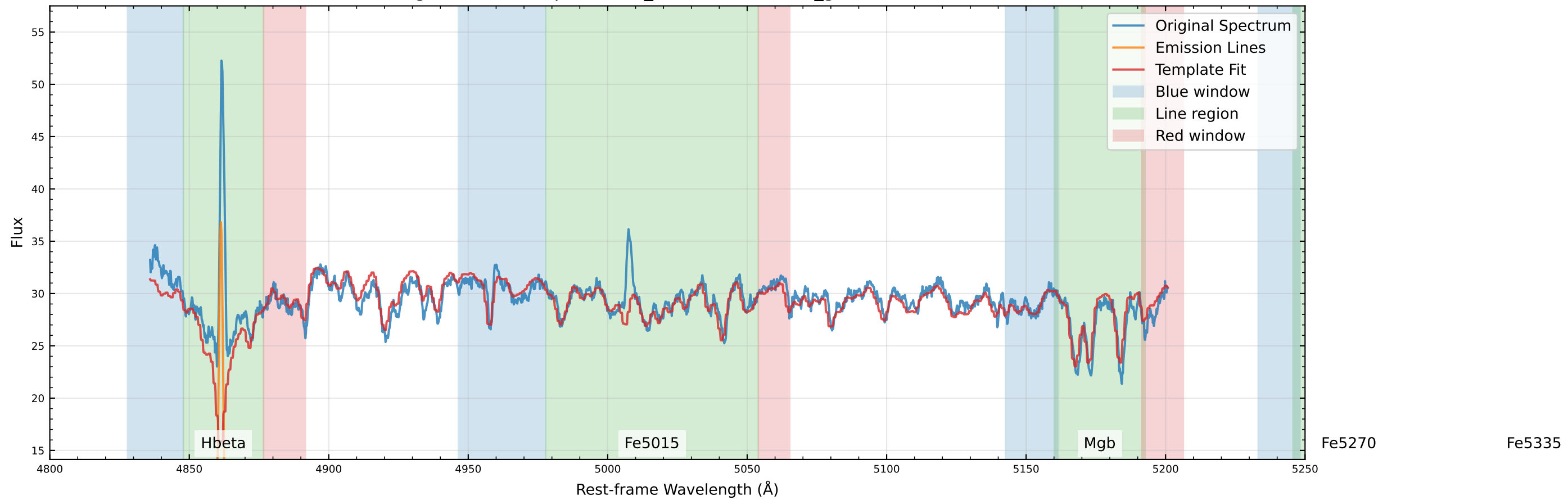
Original Data Comparison (v_star=30.7 km/s, v_gas=28.3 km/s)
