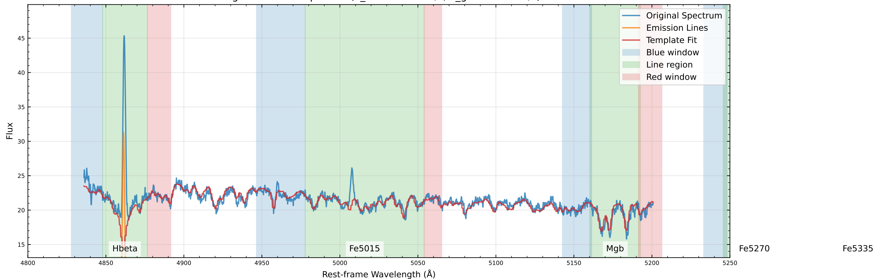
Original Data Comparison (v_star=29.7 km/s, v_gas=27.1 km/s)
